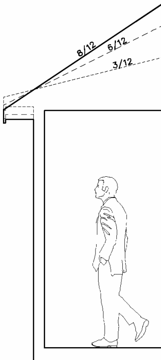
Roof Pitches
